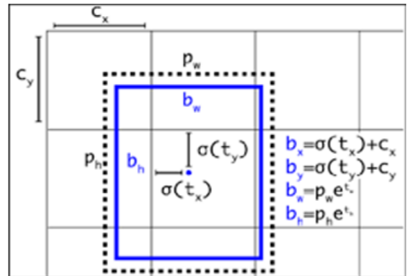
Fig. 1. Bounding boxes with location prediction and dimension priors. The height and width of the box is predicted as offsets from cluster centroids. The center coordinates of the box are predicted relative to the location of filter application using a sigmoid function.
