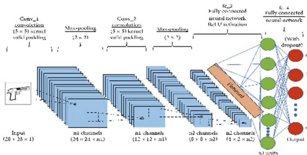
Fig. 2. Feed forward convolutional neural network (CNN).
